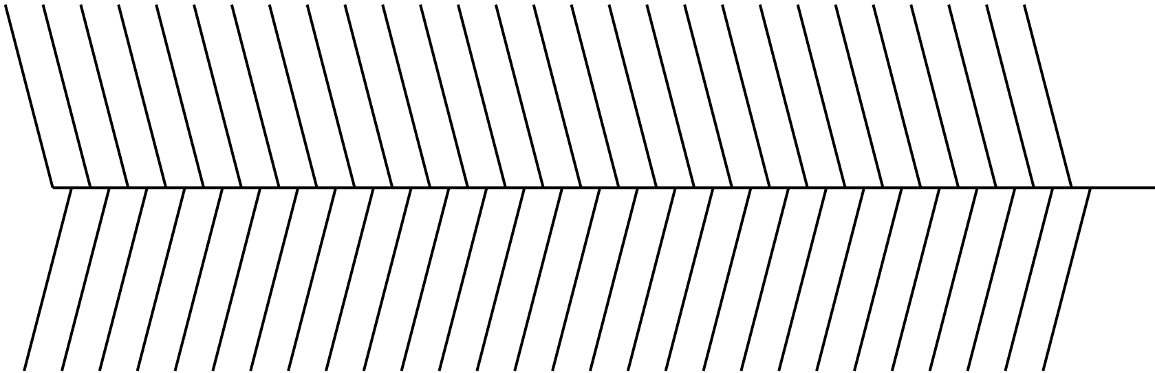
Crosscut handsaw fleam guide (fold on horizontal line) Fleam angle: 15 degrees
